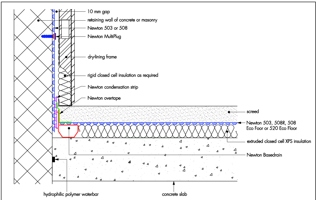
Figure 2 Installation detail
