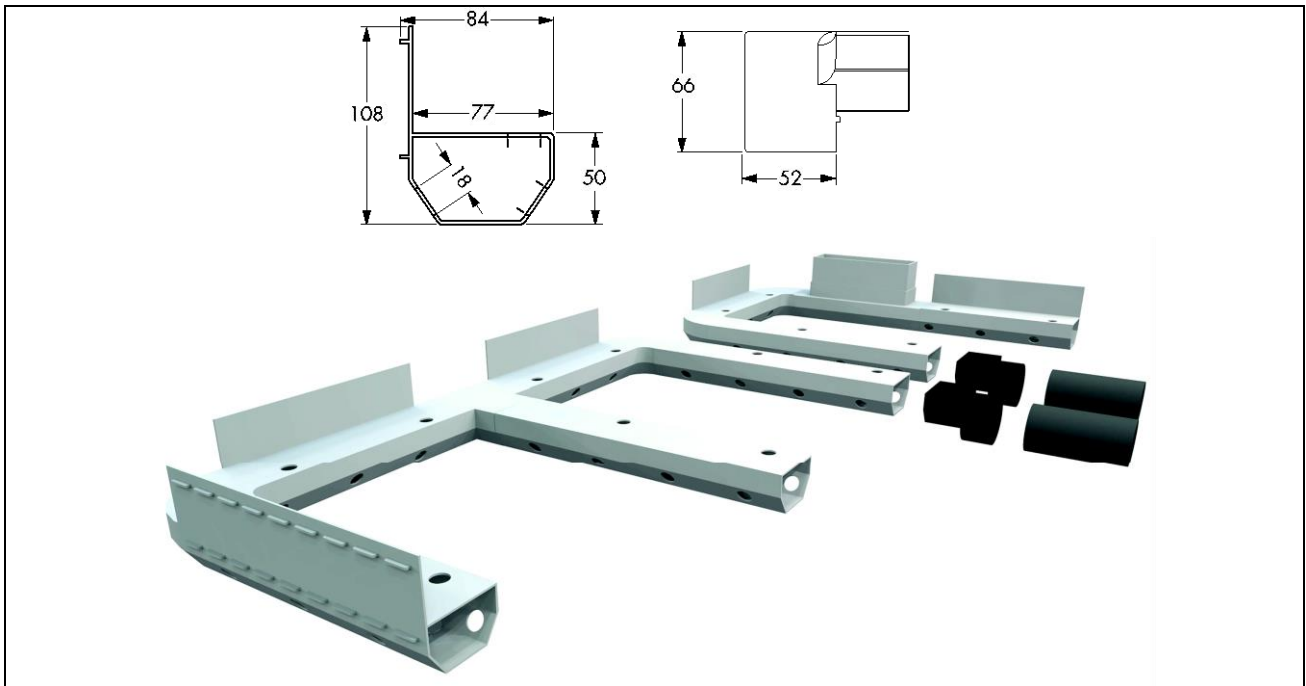
Figure 1 Newton Basedrain (all dimensions in mm)
