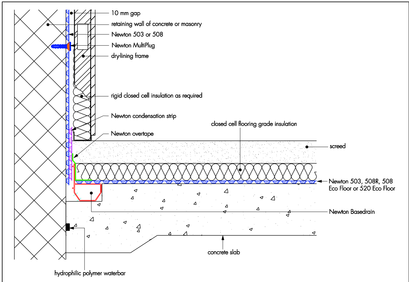
Figure 3 Installation detail
